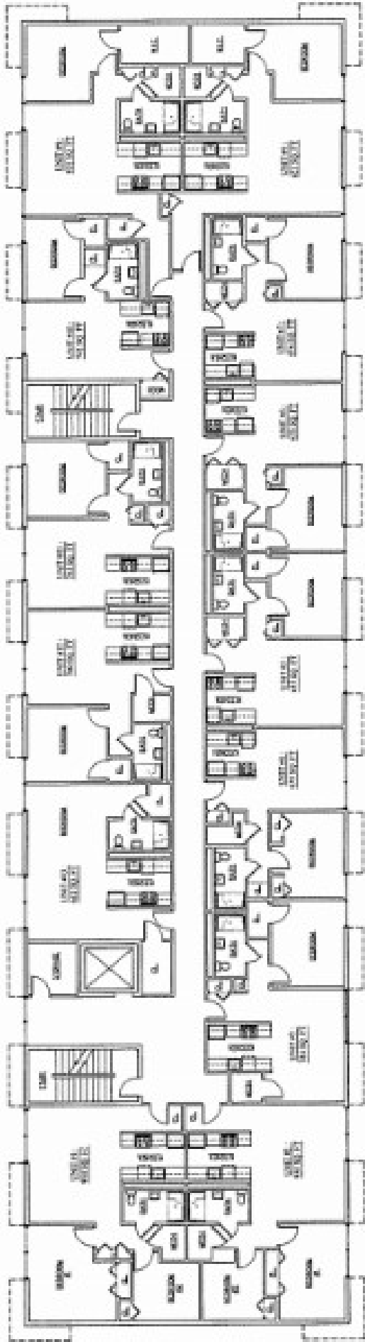
EXISTING 2ND FLOOR PLAN
