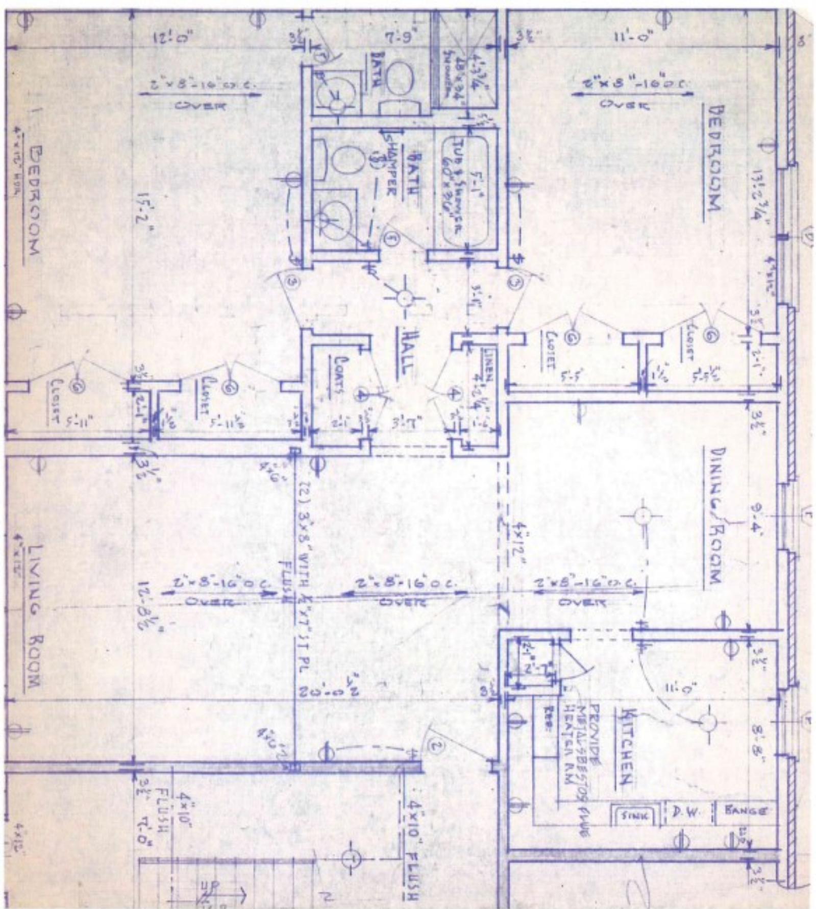
Brentwood Manor - 2 Bedroom - 1 st fl.
